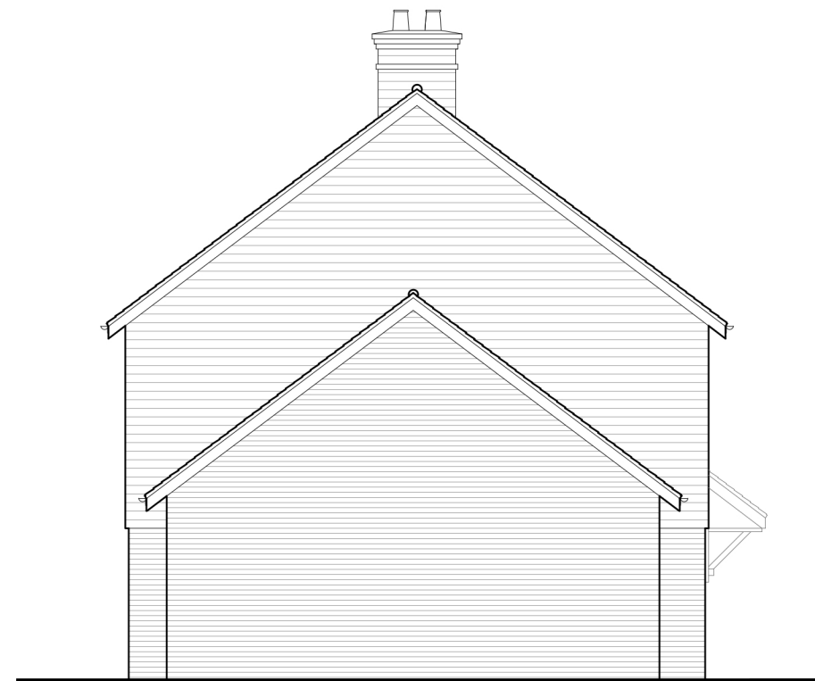
SIDE ELEVATION 2
