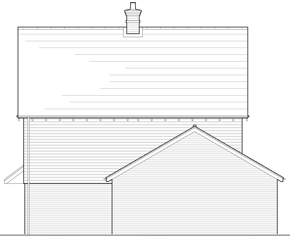
SIDE ELEVATION 1
