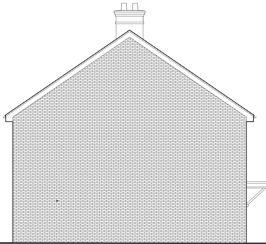
SIDE ELEVATION 2
