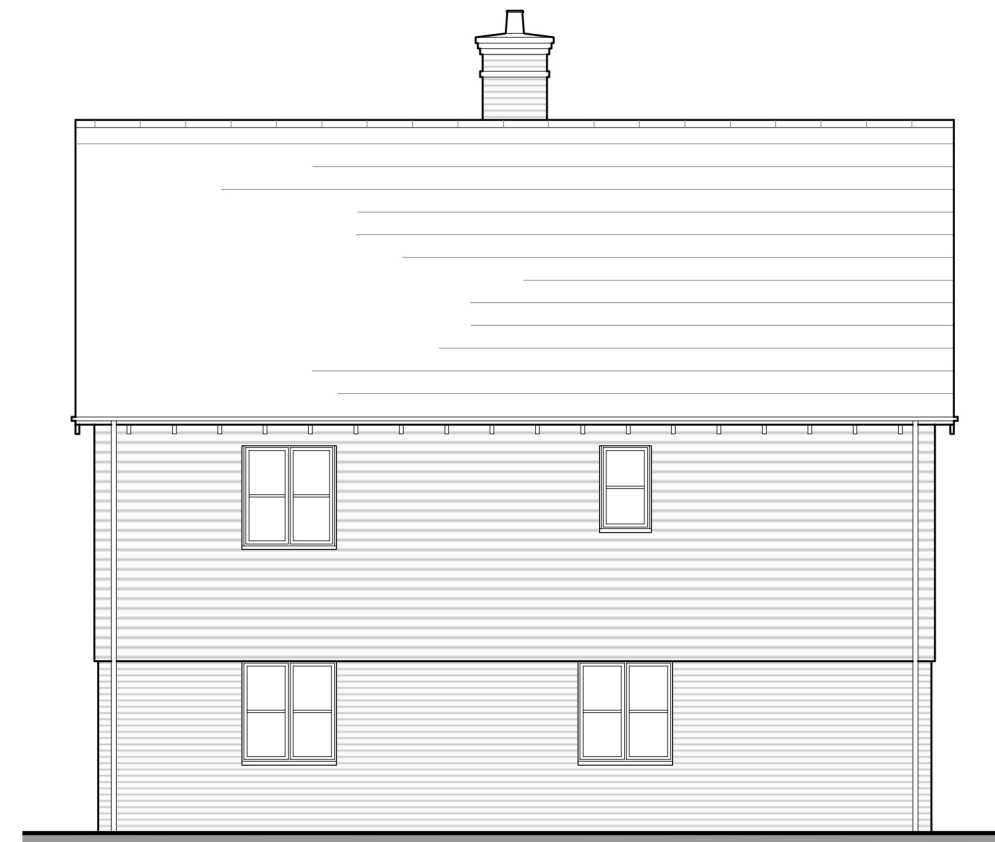
SIDE ELEVATION
