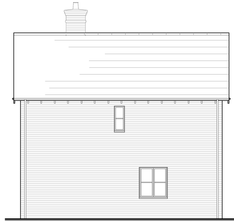
SIDE ELEVATION 2
